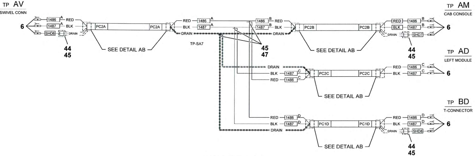
CABLE DETAIL PC2
