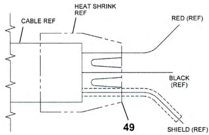
DETAIL AB CABLE ENDS TYP-BOTH ENDS
